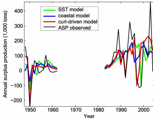
Fig. 8. Observed and modeled surplus production in the Pacific sardine population for two periods (1948-1962 and 1983-2004). The surplus production model incorporating curl-driven upwelling produced the best fit to observed production during both periods of stock assessment. Coastal upwelling and mean SST were less successful at estimating surplus production.
