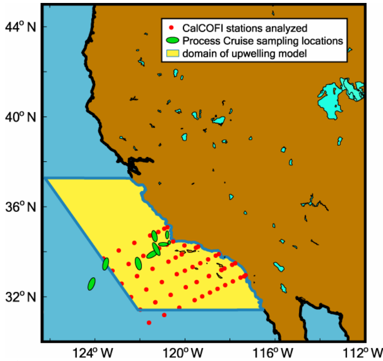
Fig. 6. Domain of the upwelling model, locations of zooplankton collections, and CalCOFI stations. The domain of the upwelling model is from Ensenada, Baja California to Santa Cruz, CA and extends \approx 300 km offshore. Each process cruise station was occupied for 3-5 days, and zooplankton was collected between dusk and dawn.
