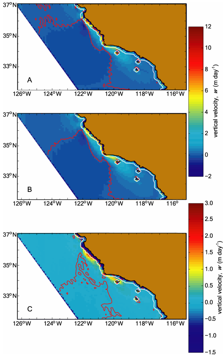
Fig. 7. Upwelling in the CCE. Wind-stress curl and coastal, alongshore winds were used to estimate mean w resulting from coastal upwelling and curl-driven upwelling in May, June, and July during 1950-1959 (A), 1990-1999 (B), and the difference in upwelling between the two periods (1990-1999 minus 1950-1959, C). The zero contour is noted by the red line. The white line along the coast separates the domains of coastal upwelling and curl-driven upwelling. Note the increase in curl-driven upwelling and the decrease in coastal upwelling in the 1990s relative to the 1950s.
